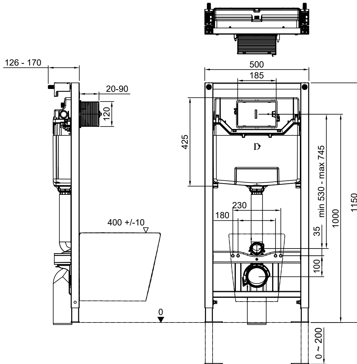
DOLPHIN SOLUTIONS LIMITED STANDARD CONCEALED WC CISTERN FRAME DB597
