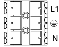
Detail X
