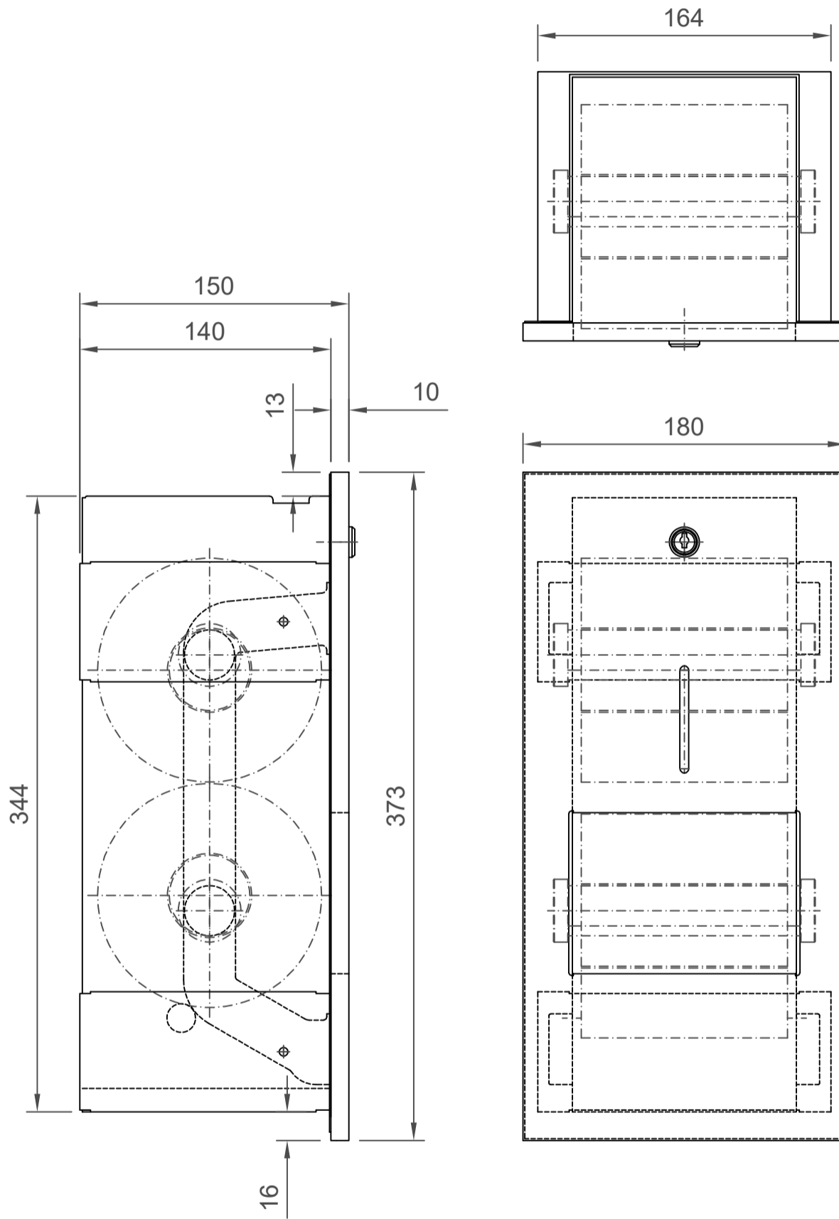
DOLPHIN SOLUTIONS LIMITED PRESTIGE RECESSED TOILET PAPER DISPENSER DP2302
