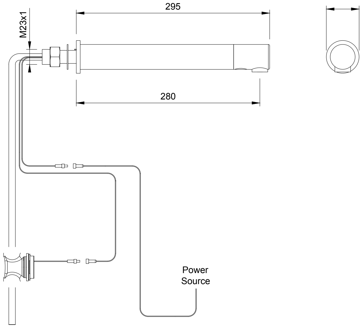
DOLPHIN SOLUTIONS LIMITED DOLPHIN BLUE PANEL MOUNTED ELECTRONIC INFRARED TAP EXTRA LONG SERIES DBXL400C / DBXL400S / DBXL425C / DBXL425S
